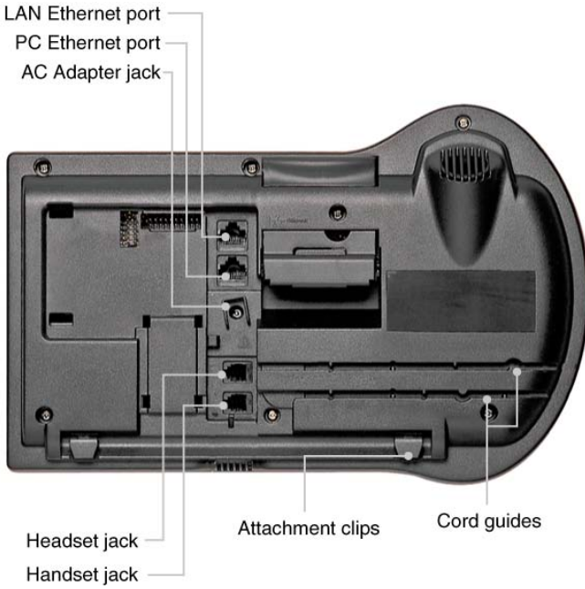
Figure 4: IP Phone connections
